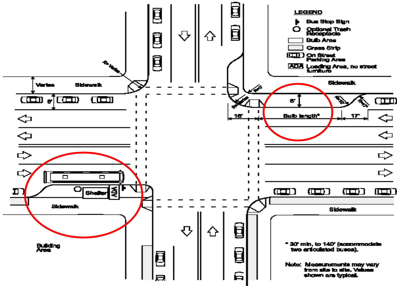
Figure 37. Typical dimensions for a bus bulb.
